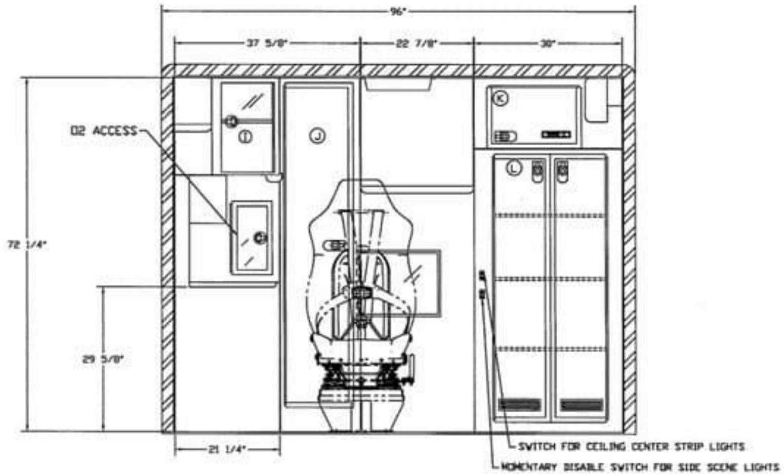
FRONT VIEW
