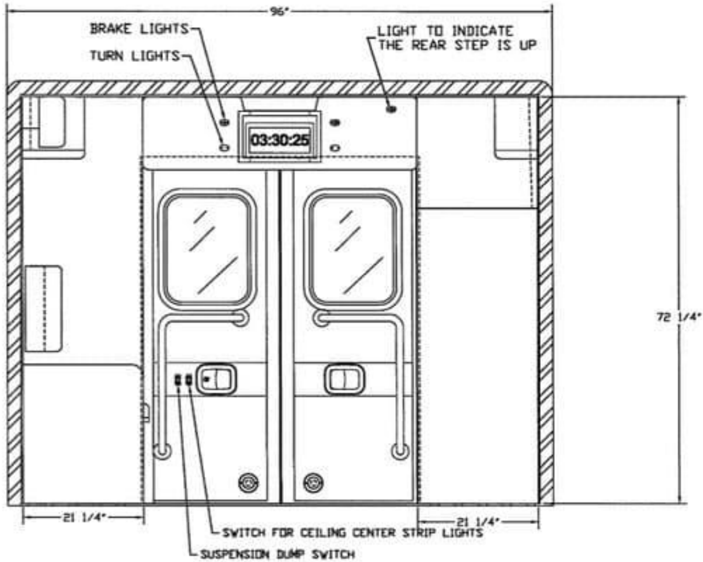
REAR VIEW
