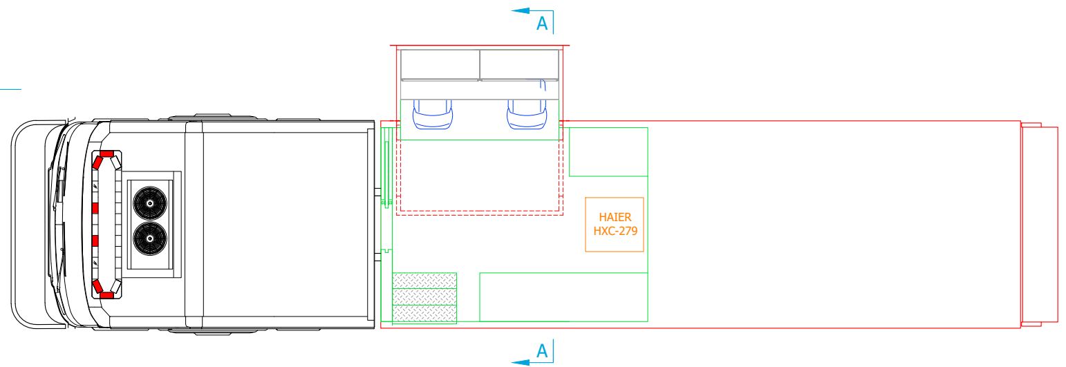
PLAN VIEW
