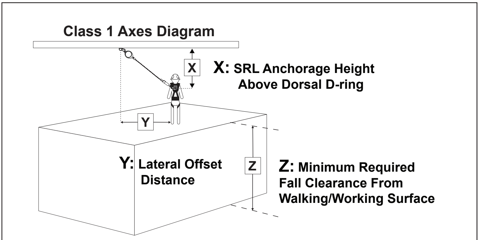
FIGURE 1 - CLASS 1 SRL AXES DIAGRAM
