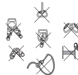
FIGURE 4 - INAPPROPRIATE CONNECTIONS
