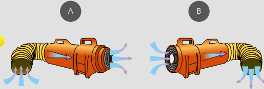
The axial blower can be attached to the canister in two positions to provide either (A) extraction or (B) ventilation.
