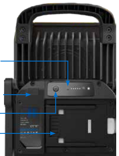
The AC adaptor also serves as the battery charger
