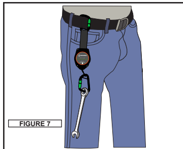
SW431 and SW432 elasticated lanyards are offered in 35 lbs capacity 50" to 62" length SW433 and SW434 elasticated lanyards are offered in 80 lbs capacity 66.5" to 80.5" length
