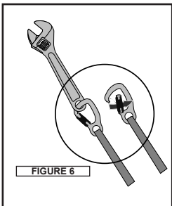
SW431 and SW432 elasticated lanyards are offered in 35 lbs capacity 50" to 62" length SW433 and SW434 elasticated lanyards are offered in 80 lbs capacity 66.5" to 80.5" length
