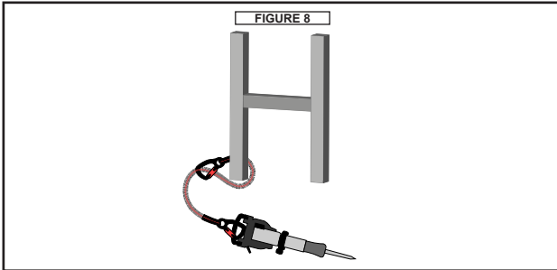
SW431 and SW432 elasticated lanyards are offered in 35 lbs capacity 50" to 62" length SW433 and SW434 elasticated lanyards are offered in 80 lbs capacity 66.5" to 80.5" length
